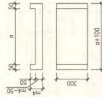
A9型烧制块
